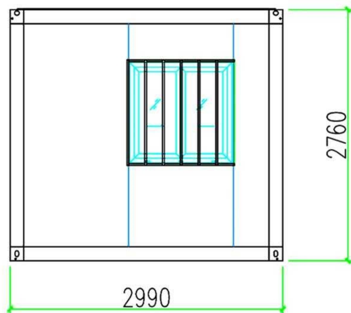
back elevation
